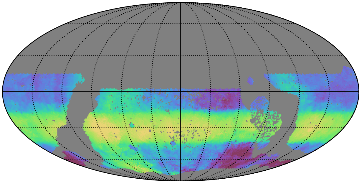
too_ignore_100_4v3.4_10yrs WFD r band: Median HA
