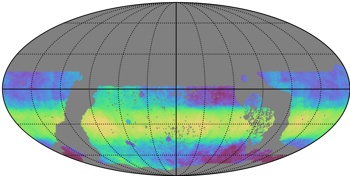
too_ignore_100_4v3.4_10yrs WFD i band: Median HA
