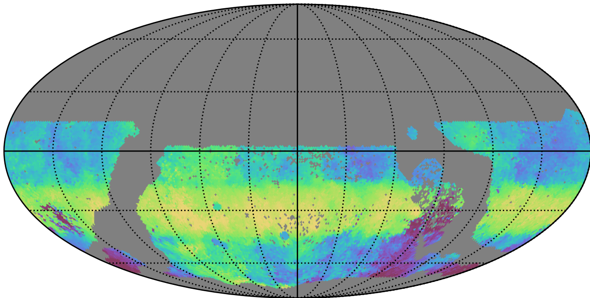
too_ignore_100_4v3.4_10yrs WFD g band: Median HA
