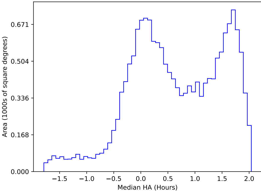
too_ignore_100_4v3.4_10yrs WFD g band: Median HA
