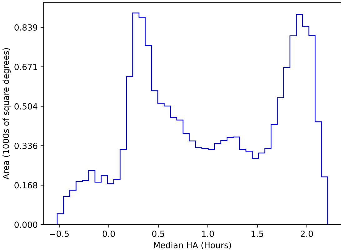
too_ignore_100_4v3.4_10yrs WFD all bands: Median HA
