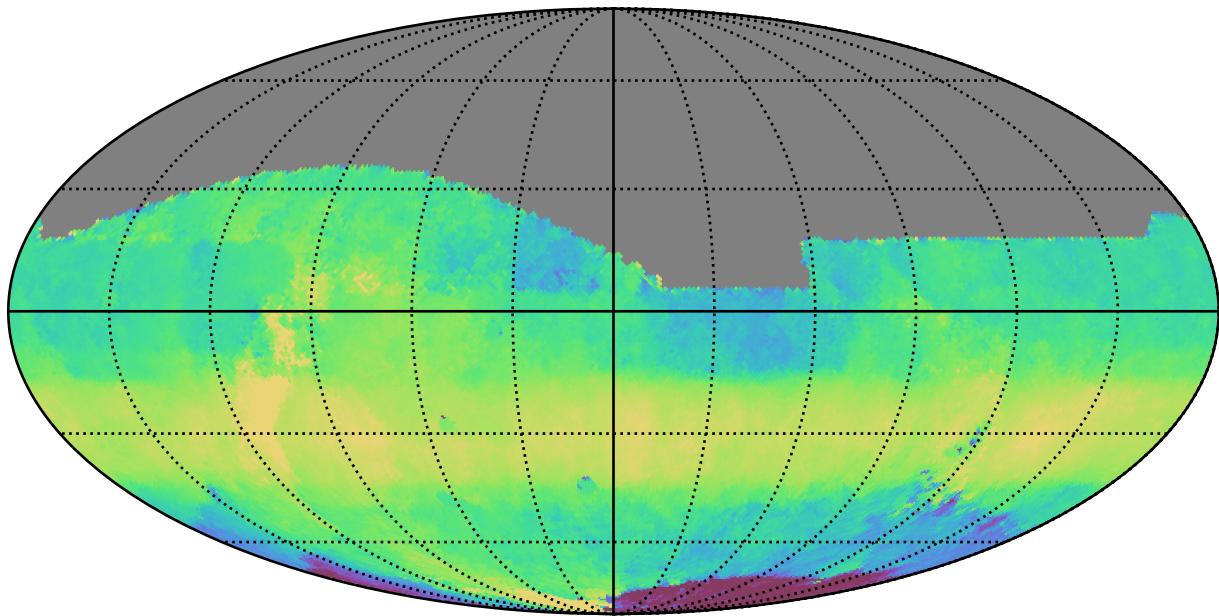
too_ignore_100_4v3.4_10yrs All sky z band: Median HA
