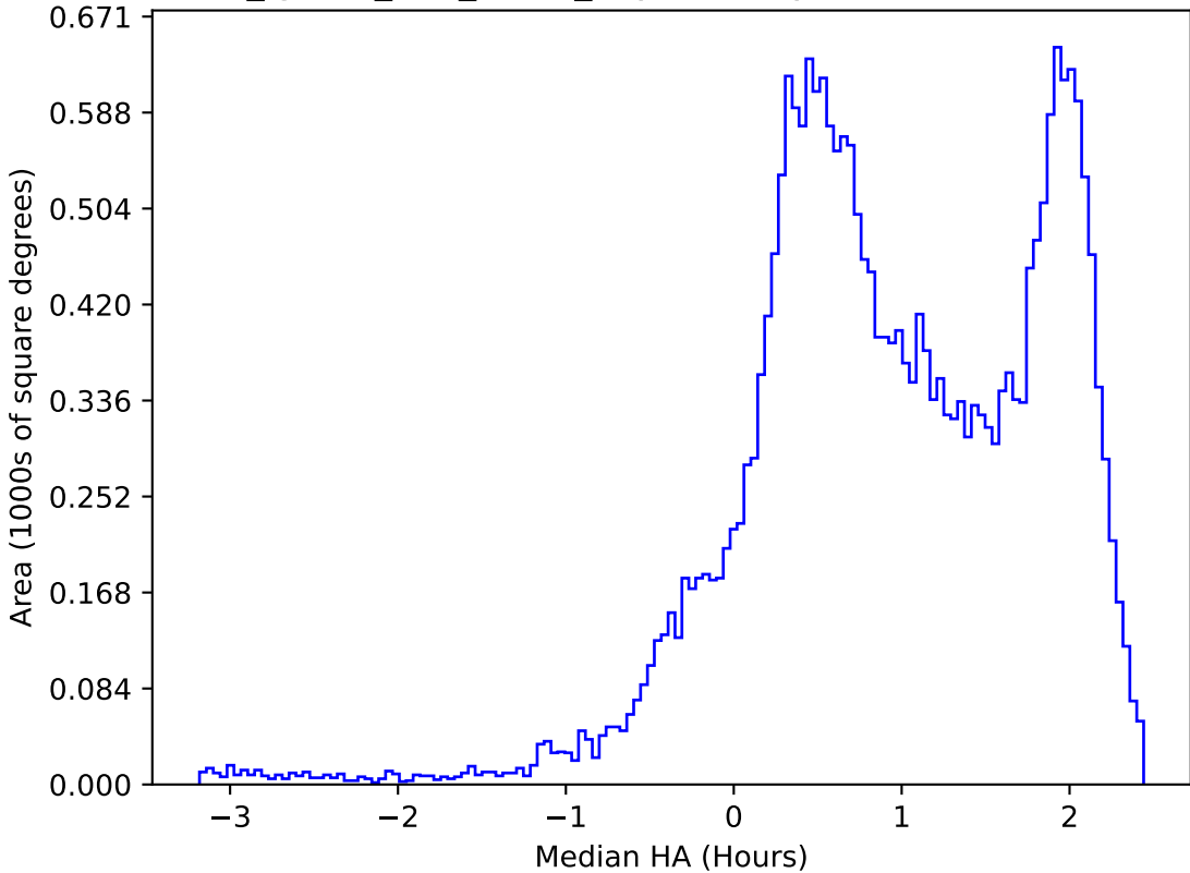
too_ignore_100_4v3.4_10yrs All sky z band: Median HA
