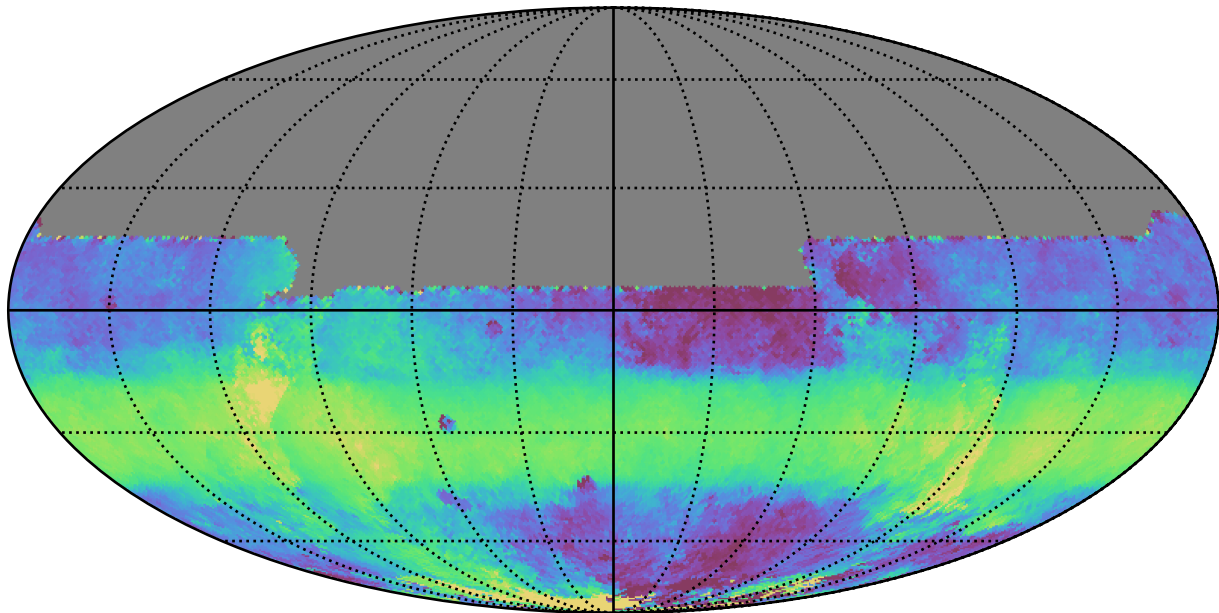
too_ignore_100_4v3.4_10yrs All sky y band: Median HA
