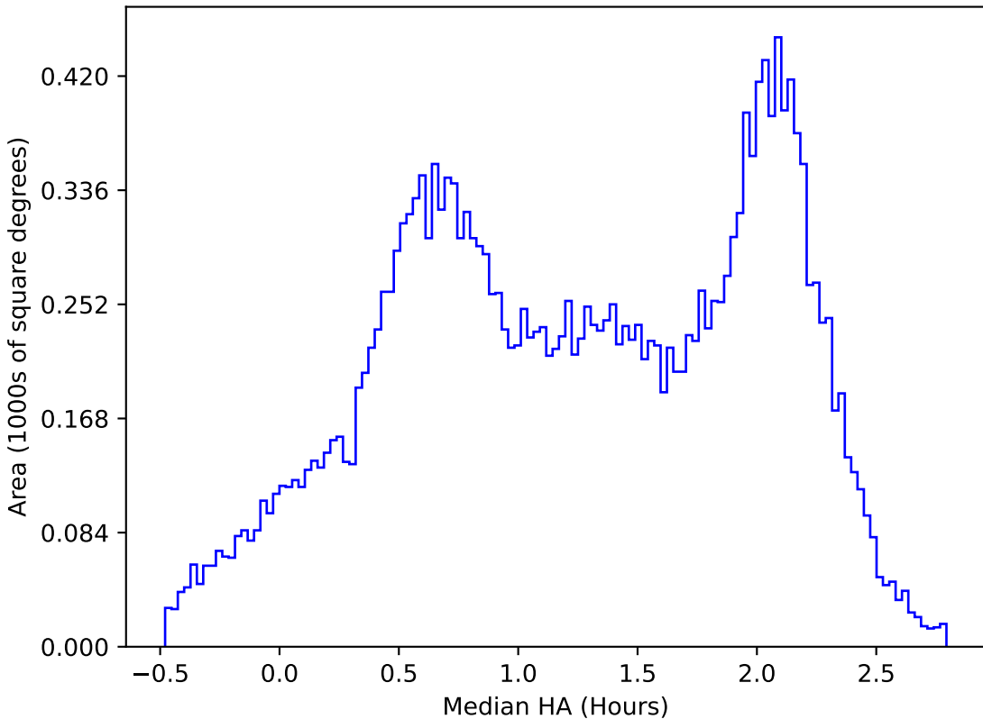
too_ignore_100_4v3.4_10yrs All sky y band: Median HA
