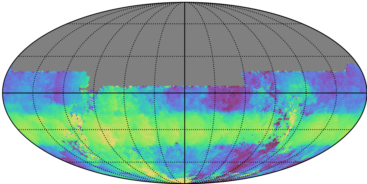
too_ignore_100_4v3.4_10yrs All sky u band: Median HA
