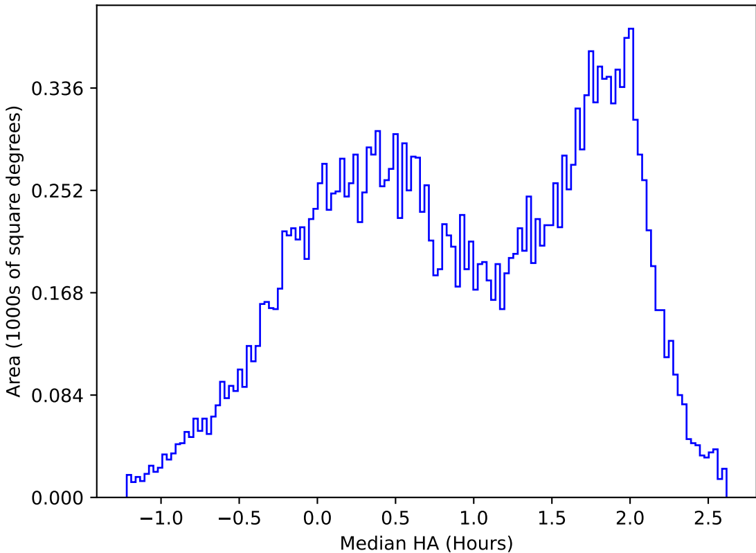
too_ignore_100_4v3.4_10yrs All sky u band: Median HA
