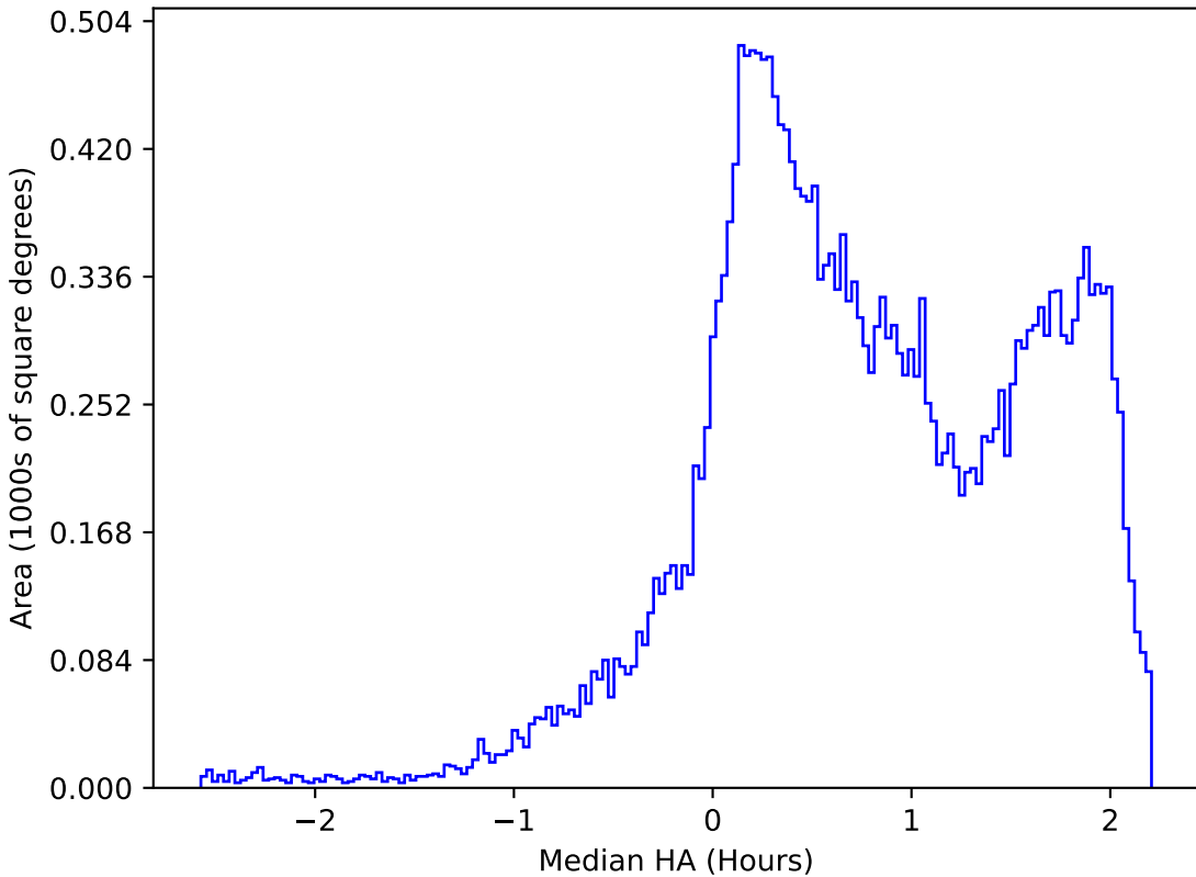
too_ignore_100_4v3.4_10yrs All sky r band: Median HA
