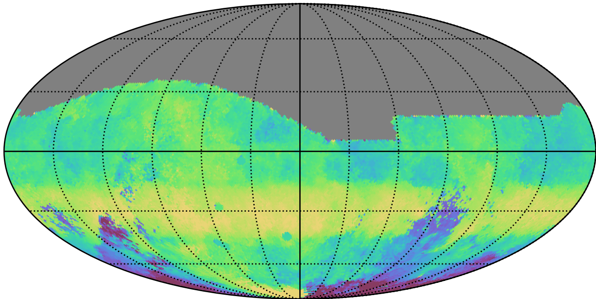
too_ignore_100_4v3.4_10yrs All sky g band: Median HA
