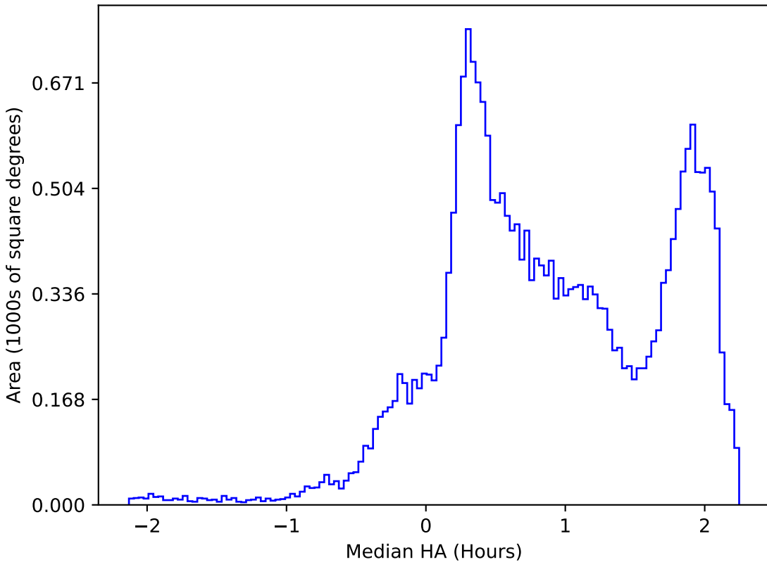
too_ignore_100_4v3.4_10yrs All sky all bands: Median HA
