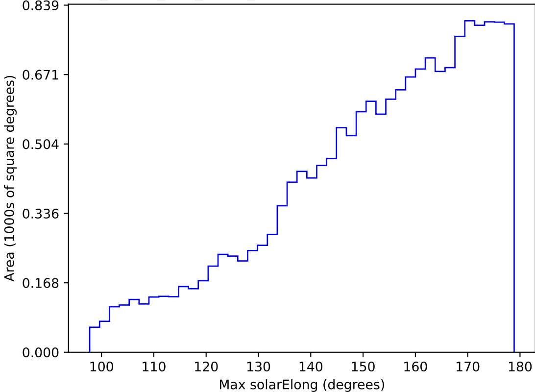
too_ignore_100_4v3.4_10yrs WFD u band: Max solarElong
