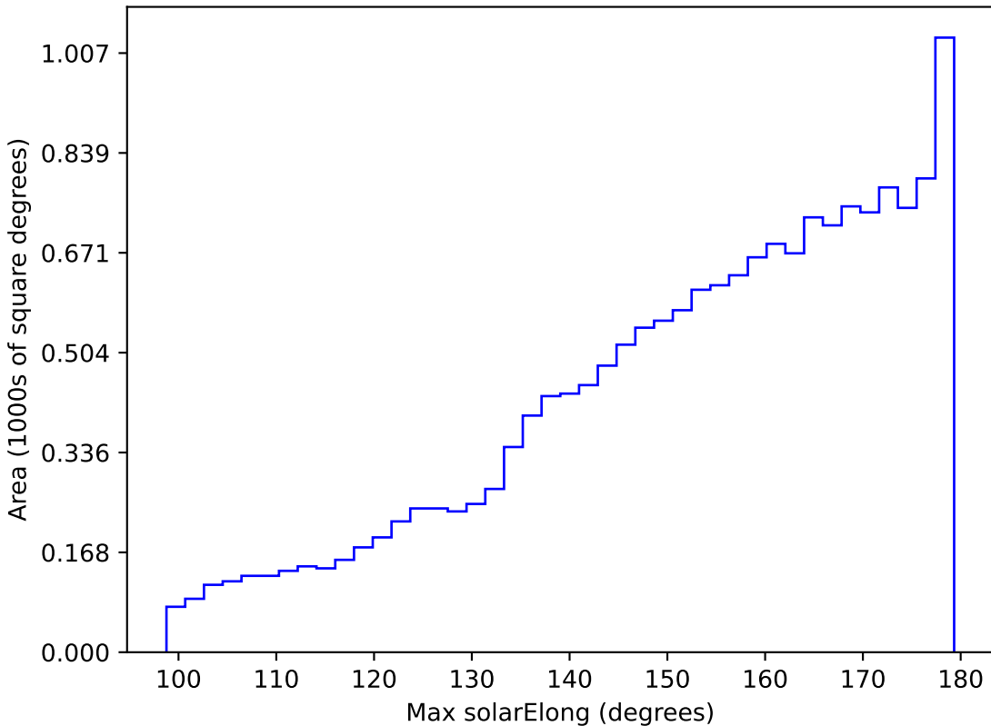
too_ignore_100_4v3.4_10yrs WFD r band: Max solarElong
