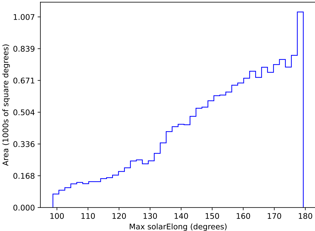
too_ignore_100_4v3.4_10yrs WFD i band: Max solarElong
