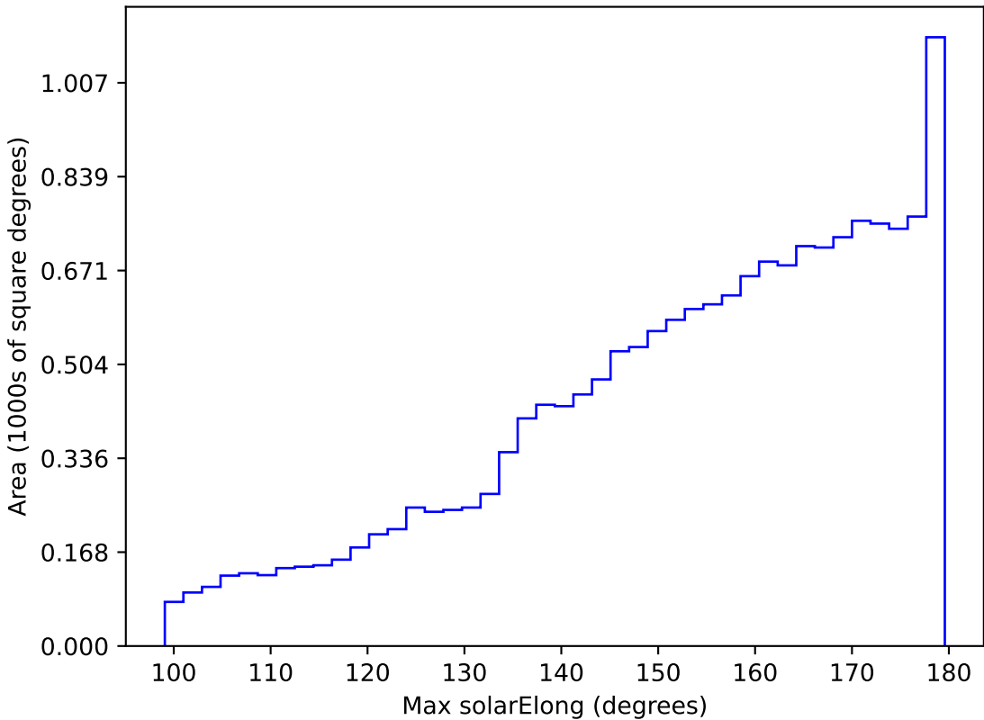
too_ignore_100_4v3.4_10yrs WFD all bands: Max solarElong
