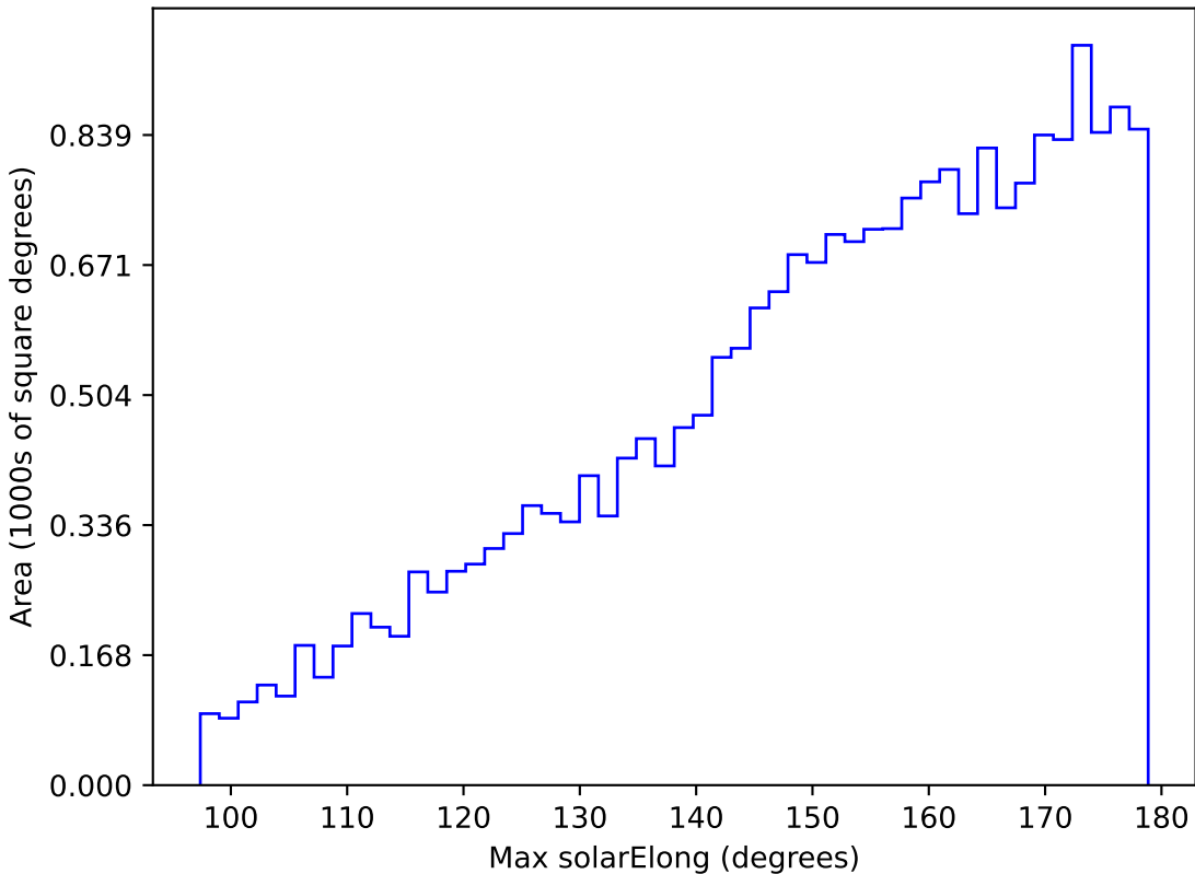
too_ignore_100_4v3.4_10yrs All sky u band: Max solarElong
