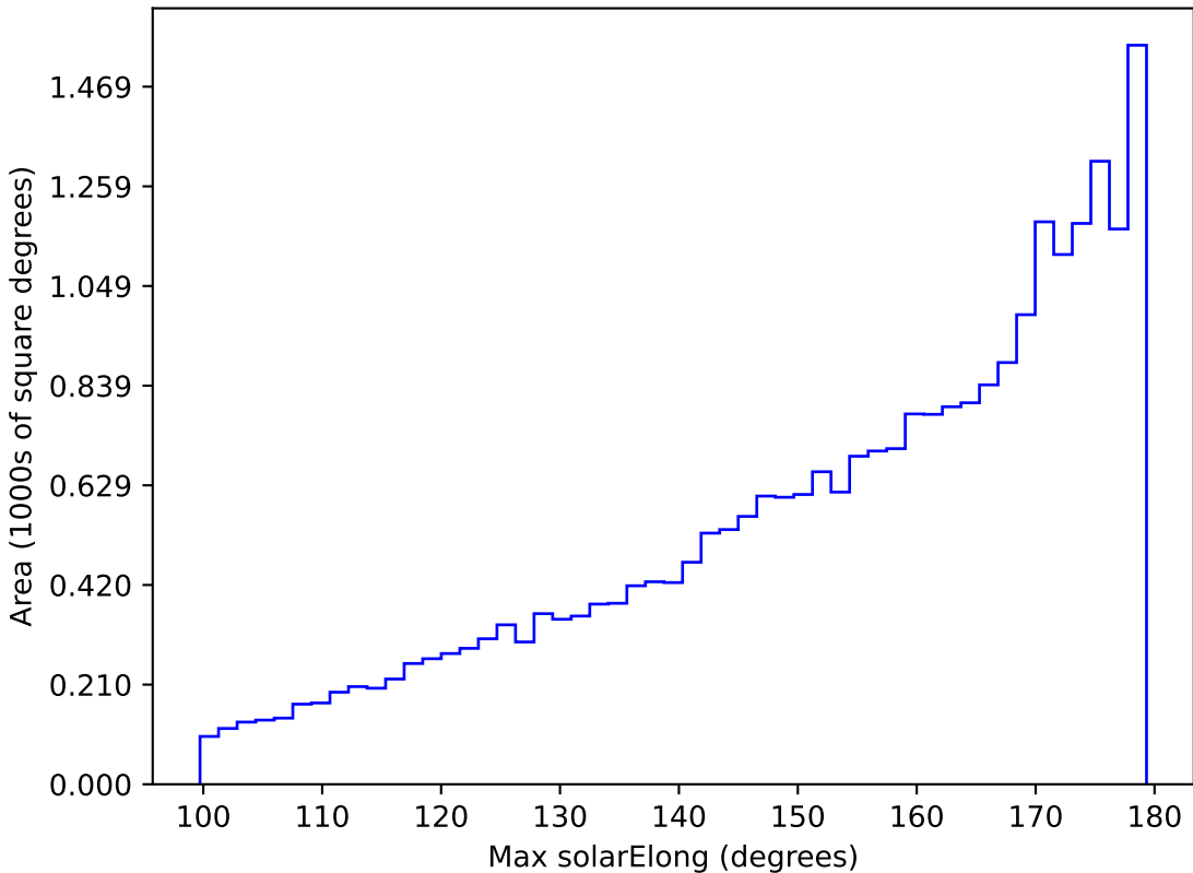
too_ignore_100_4v3.4_10yrs All sky i band: Max solarElong
