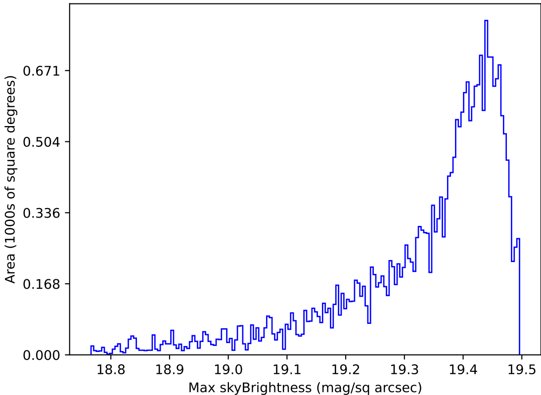
too_ignore_100_4v3.4_10yrs Yr 1 z band: Max skyBrightness
