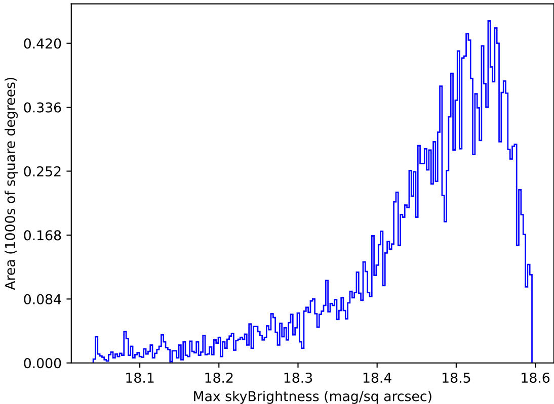
too_ignore_100_4v3.4_10yrs Yr 1 y band: Max skyBrightness
