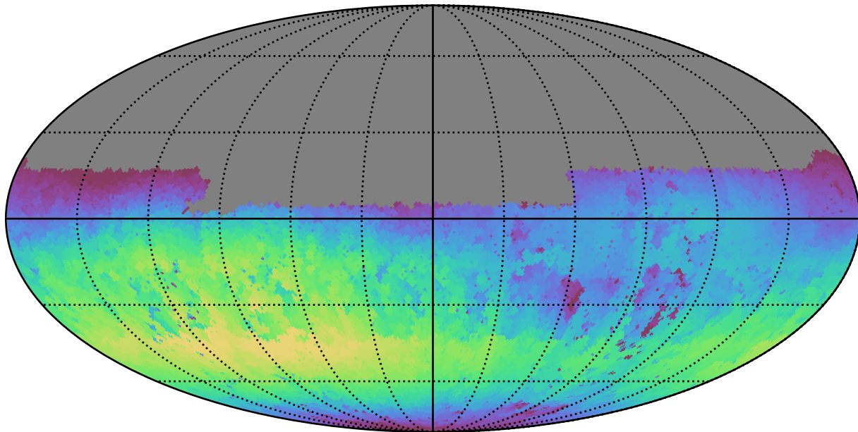
too_ignore_100_4v3.4_10yrs Yr 1 u band: Max skyBrightness
