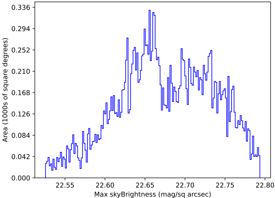
too_ignore_100_4v3.4_10yrs Yr 1 u band: Max skyBrightness
