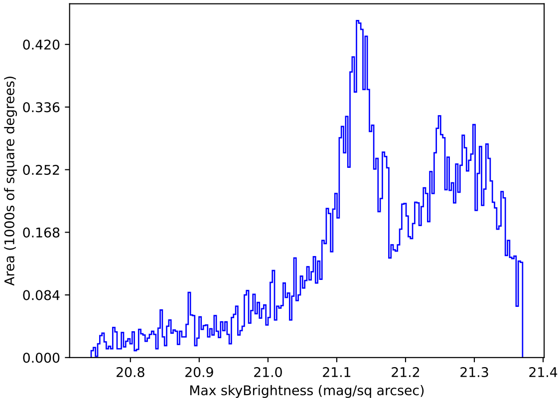
too_ignore_100_4v3.4_10yrs Yr 1 r band: Max skyBrightness
