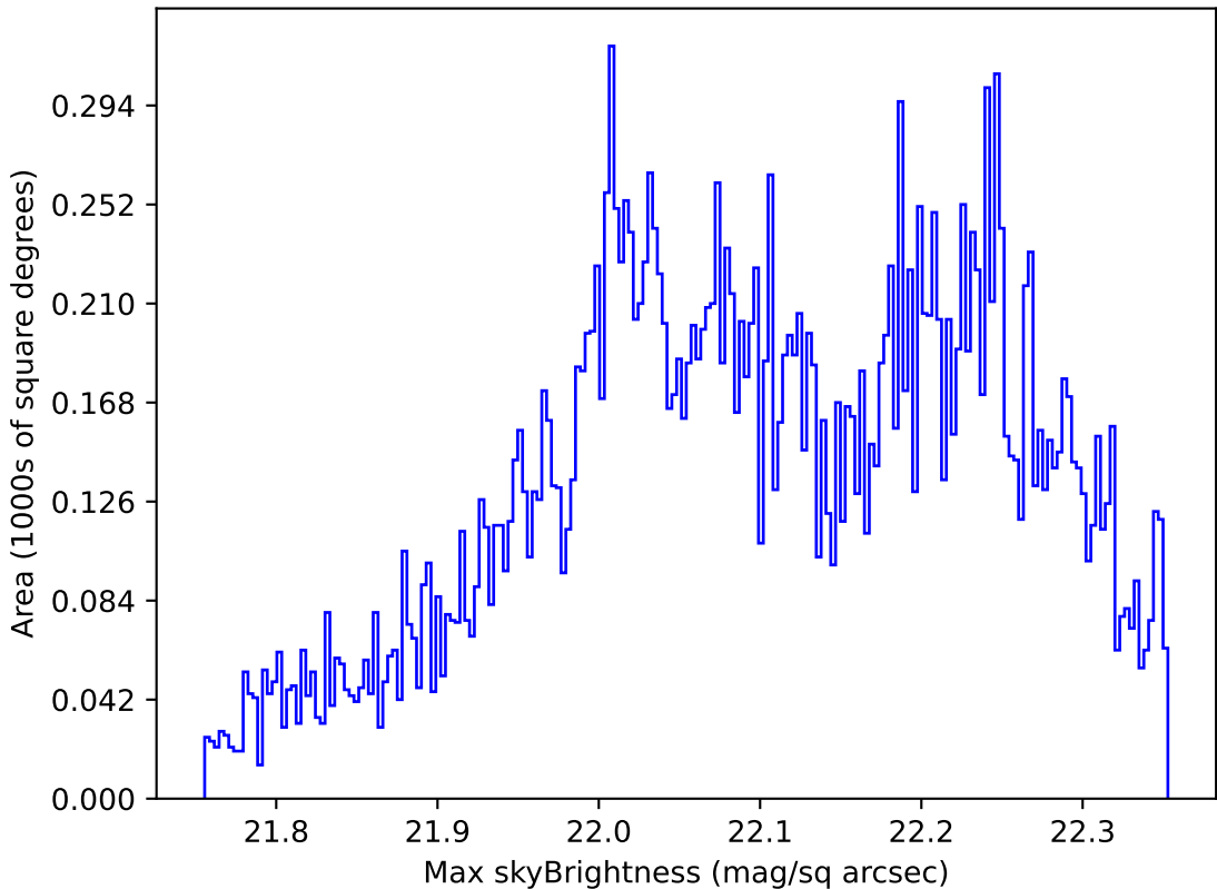
too_ignore_100_4v3.4_10yrs Yr 1 g band: Max skyBrightness
