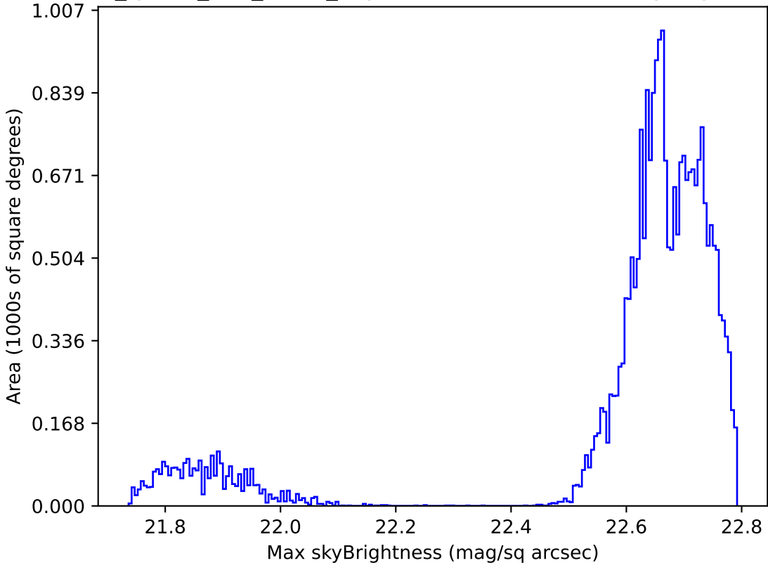
too_ignore_100_4v3.4_10yrs Yr 1 all bands: Max skyBrightness
