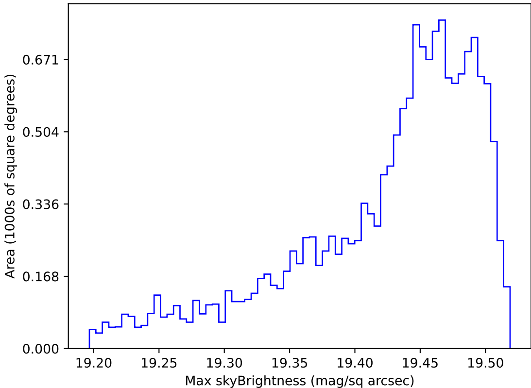
too_ignore_100_4v3.4_10yrs WFD z band: Max skyBrightness
