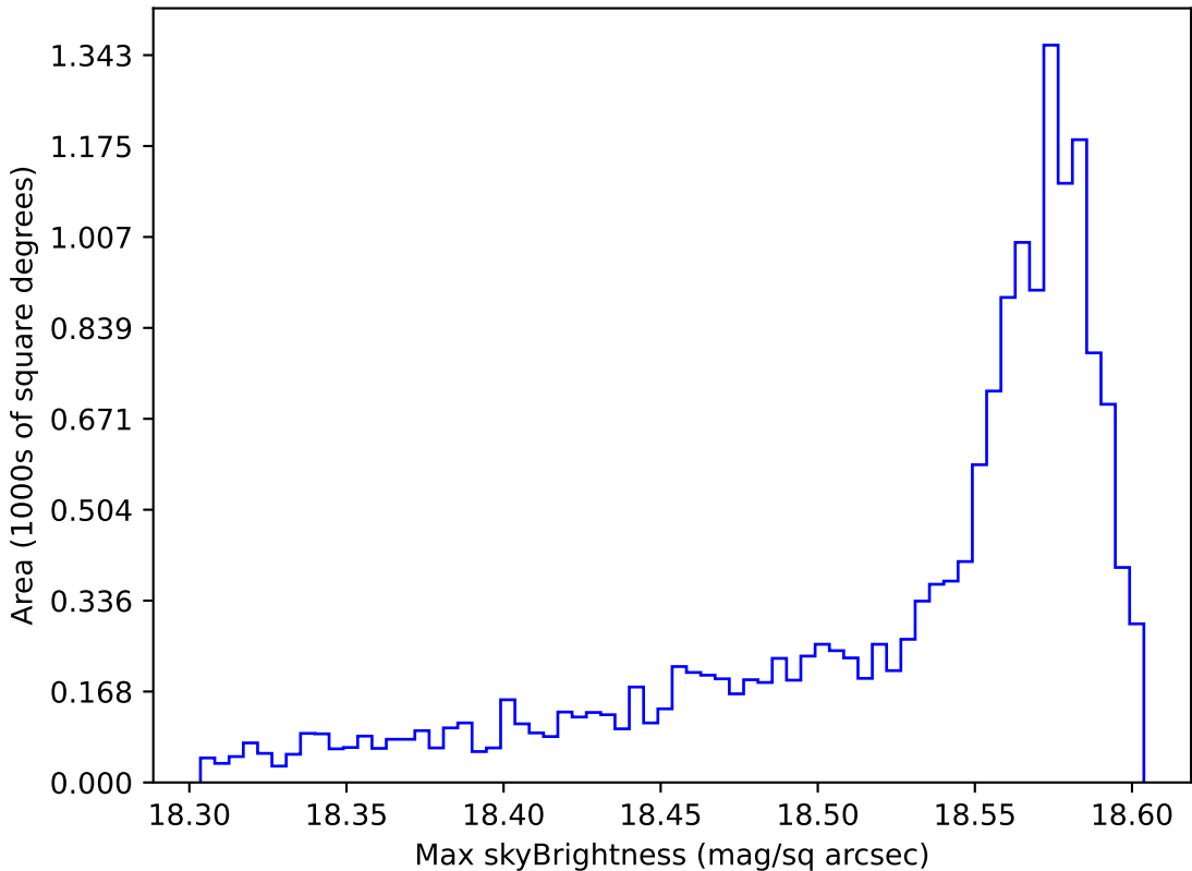
too_ignore_100_4v3.4_10yrs WFD y band: Max skyBrightness
