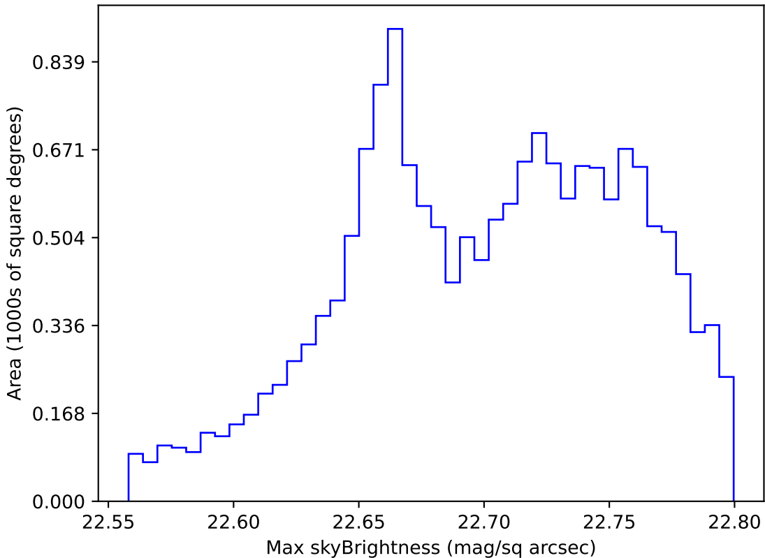
too_ignore_100_4v3.4_10yrs WFD u band: Max skyBrightness
