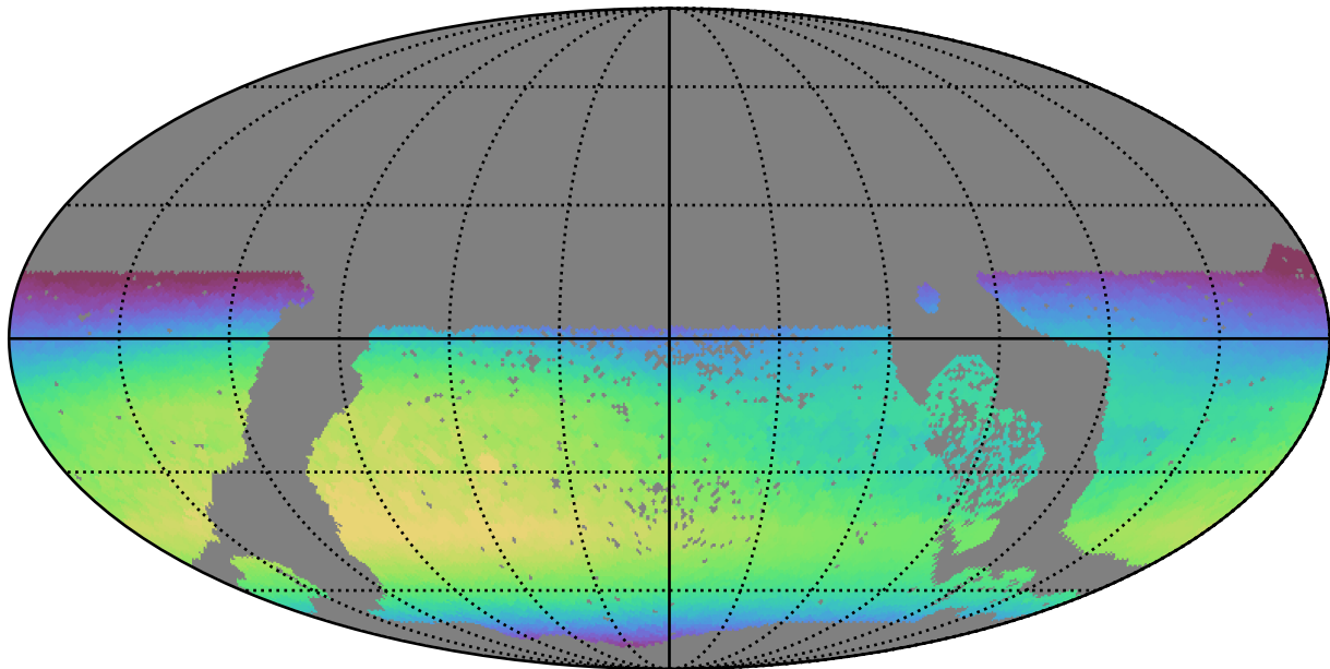
too_ignore_100_4v3.4_10yrs WFD i band: Max skyBrightness
