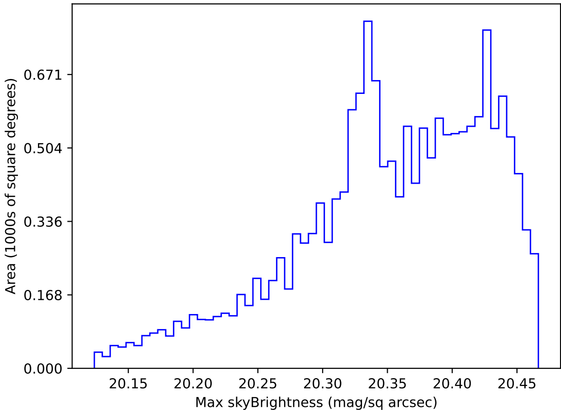
too_ignore_100_4v3.4_10yrs WFD i band: Max skyBrightness
