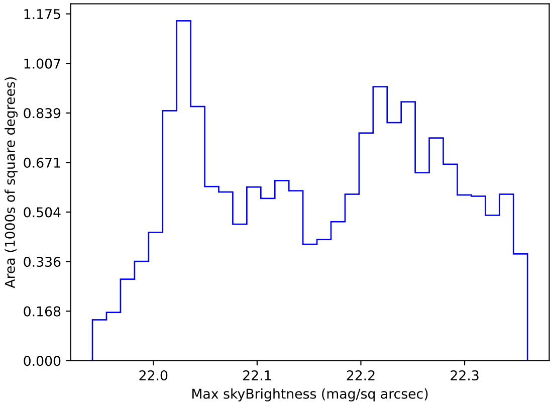
too_ignore_100_4v3.4_10yrs WFD g band: Max skyBrightness
