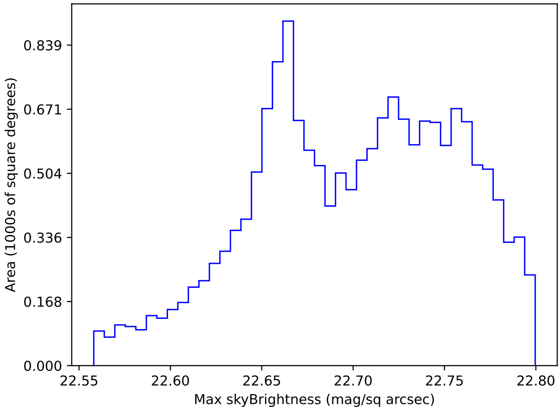
too_ignore_100_4v3.4_10yrs WFD all bands: Max skyBrightness
