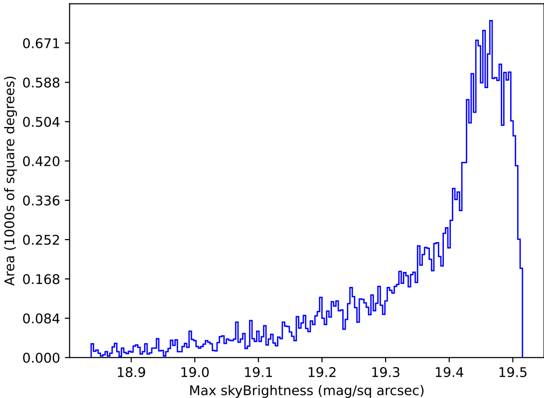
too_ignore_100_4v3.4_10yrs All sky z band: Max skyBrightness
