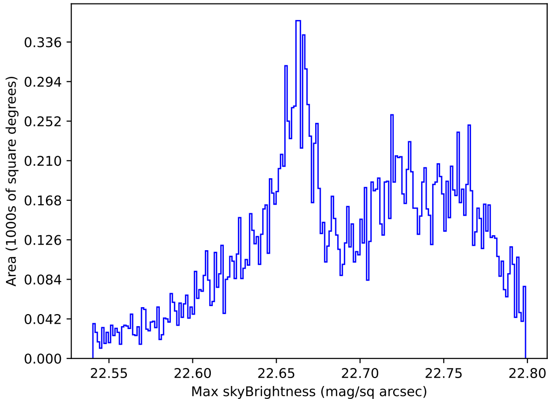
too_ignore_100_4v3.4_10yrs All sky u band: Max skyBrightness
