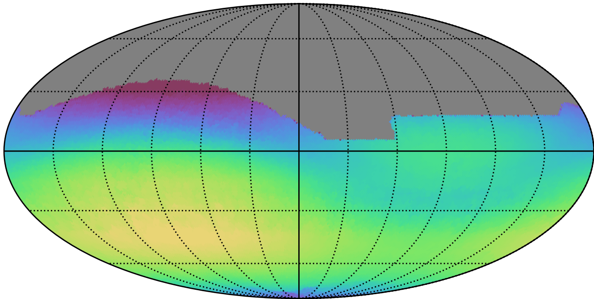
too_ignore_100_4v3.4_10yrs All sky r band: Max skyBrightness
