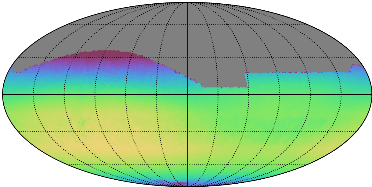
too_ignore_100_4v3.4_10yrs All sky i band: Max skyBrightness
