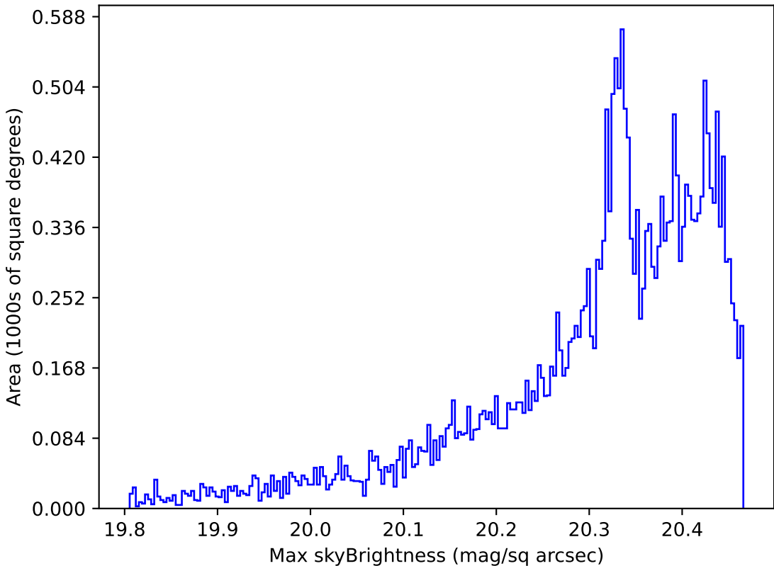
too_ignore_100_4v3.4_10yrs All sky i band: Max skyBrightness
