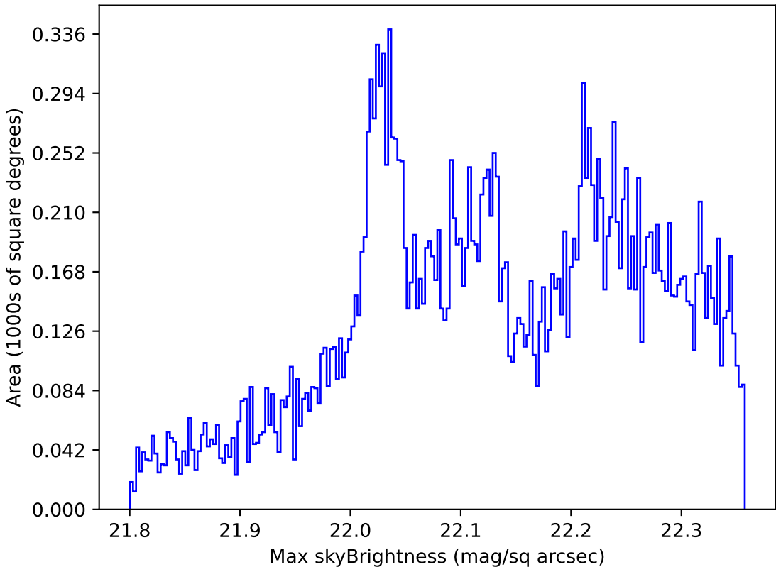
too_ignore_100_4v3.4_10yrs All sky g band: Max skyBrightness
