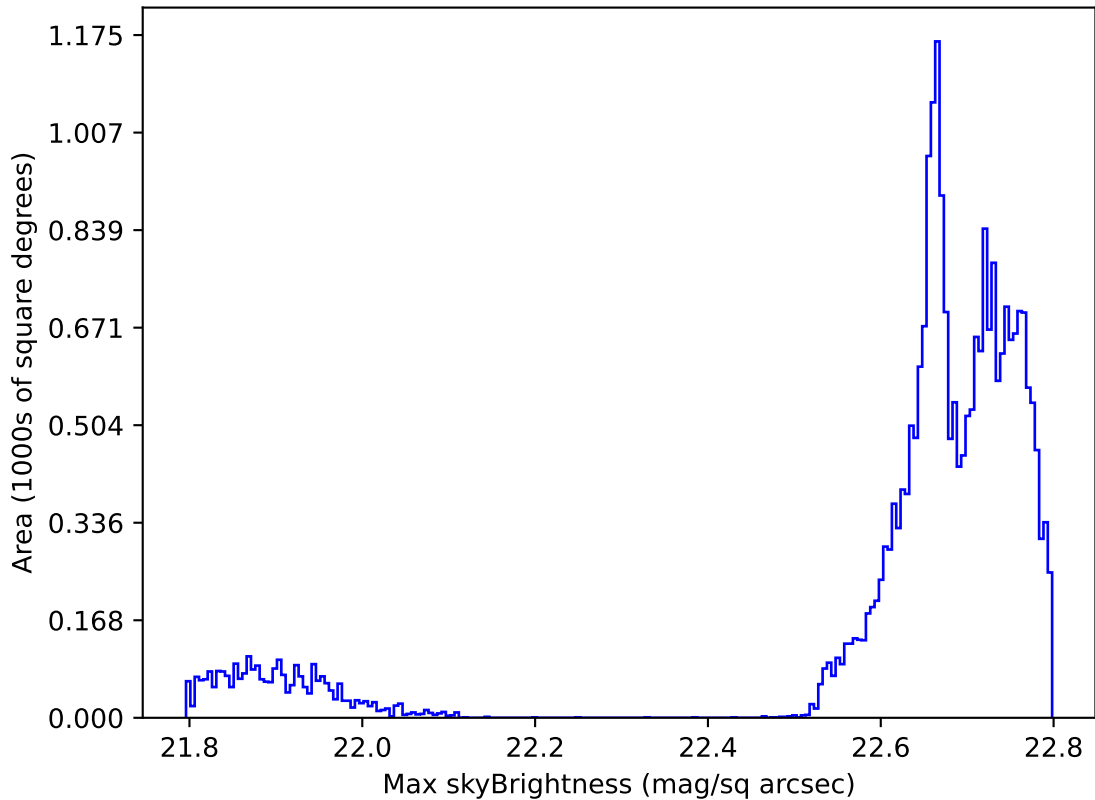
too_ignore_100_4v3.4_10yrs All sky all bands: Max skyBrightness
