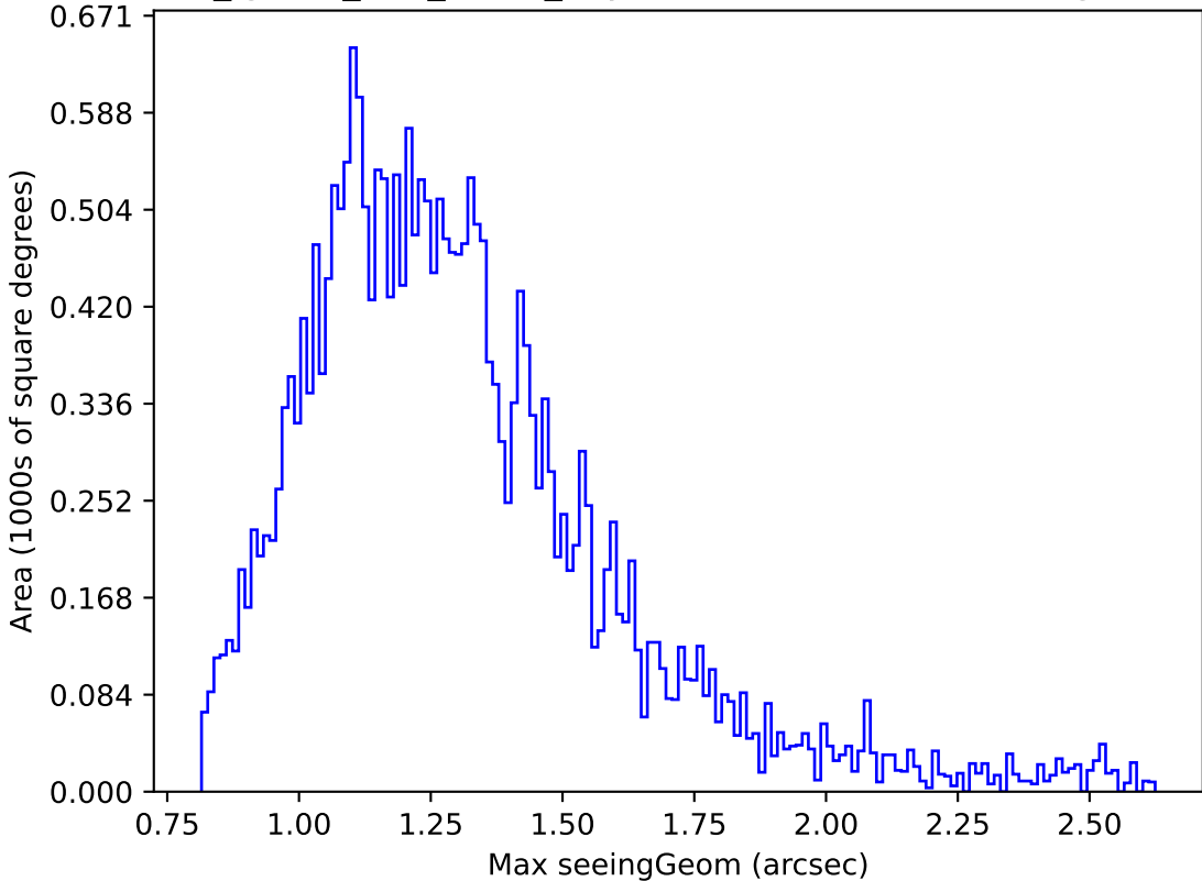
too_ignore_100_4v3.4_10yrs Yr 1 z band: Max seeingGeom
