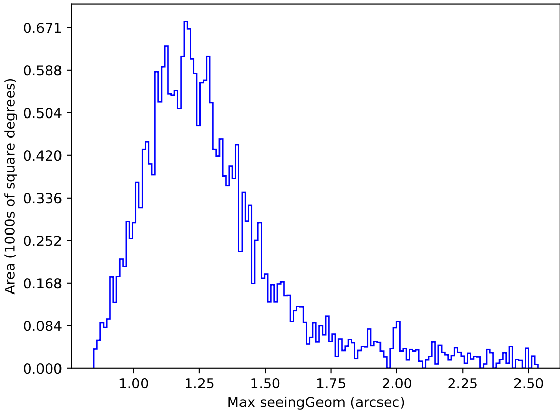
too_ignore_100_4v3.4_10yrs Yr 1 y band: Max seeingGeom
