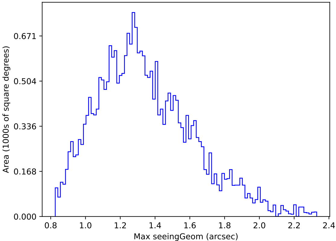
too_ignore_100_4v3.4_10yrs Yr 1 r band: Max seeingGeom
