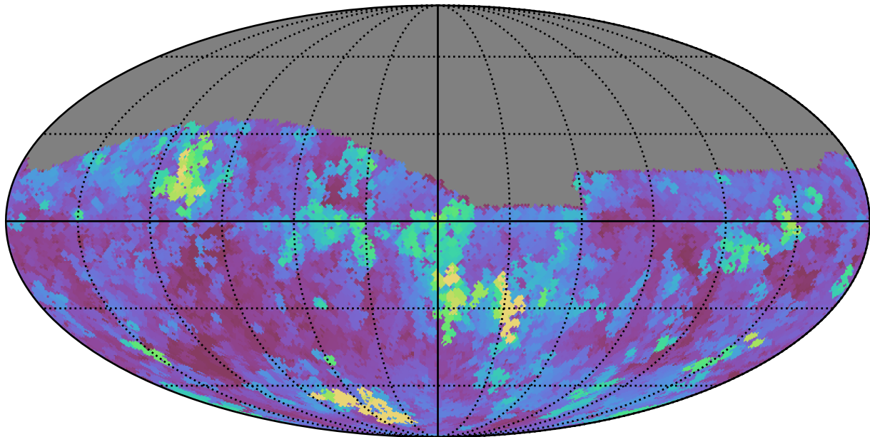
too_ignore_100_4v3.4_10yrs Yr 1 i band: Max seeingGeom
