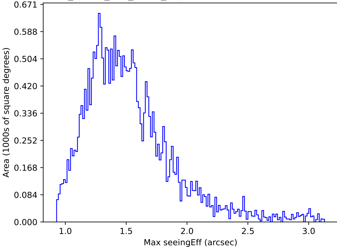
too_ignore_100_4v3.4_10yrs Yr 1 z band: Max seeingEff
