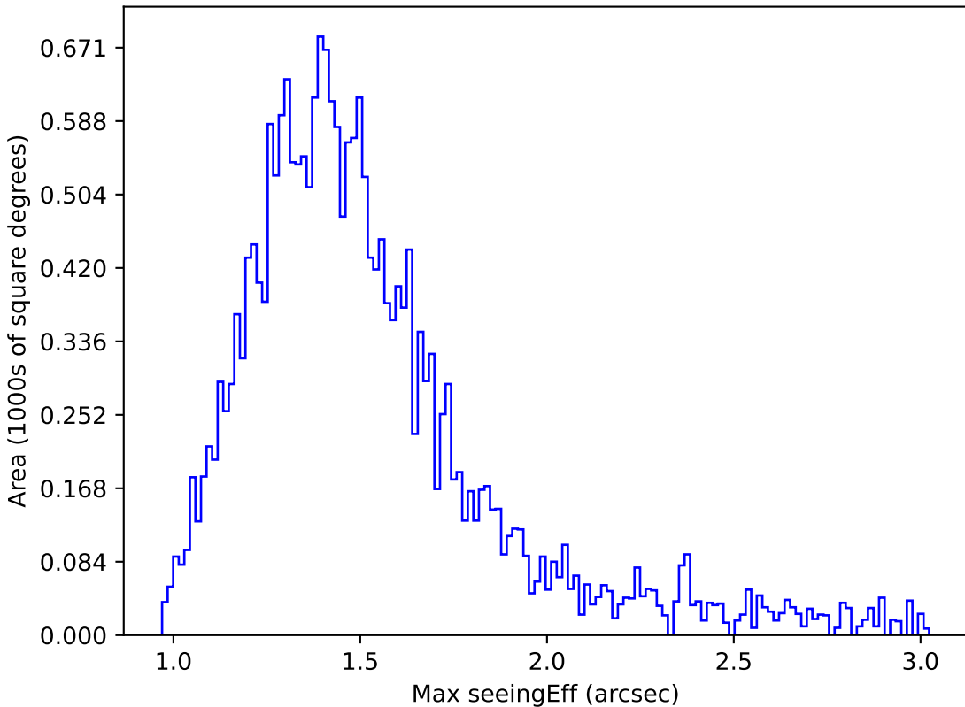
too_ignore_100_4v3.4_10yrs Yr 1 y band: Max seeingEff
