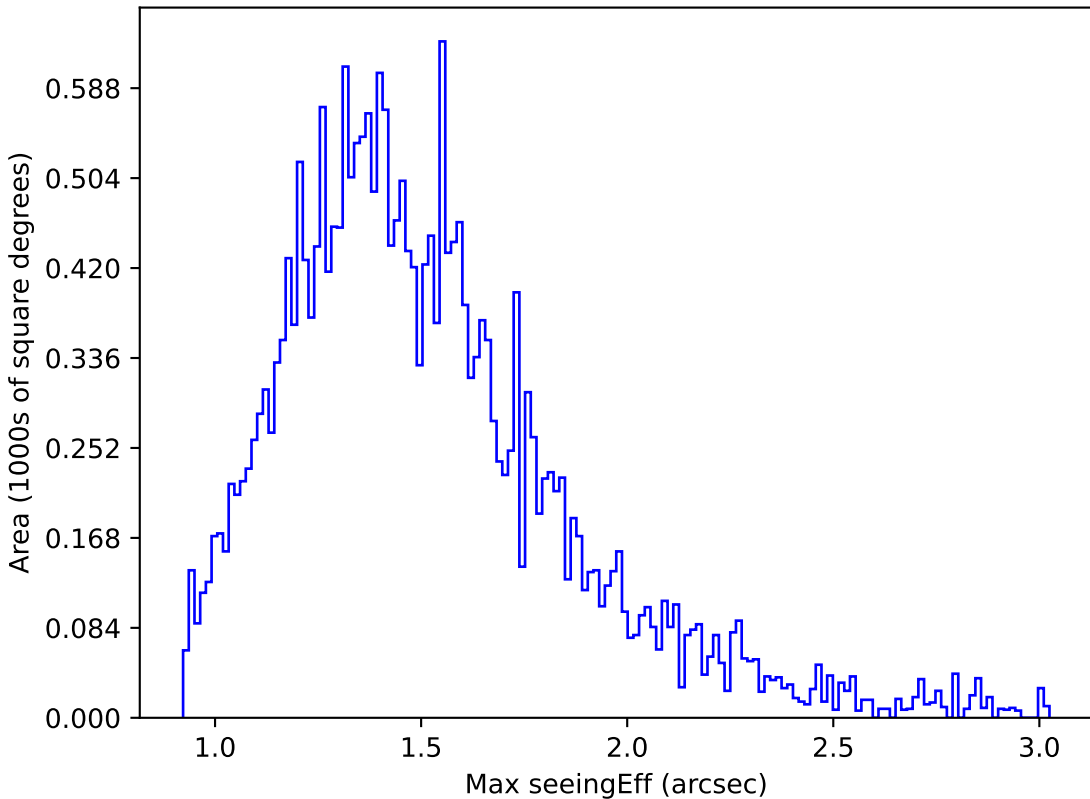
too_ignore_100_4v3.4_10yrs Yr 1 i band: Max seeingEff
