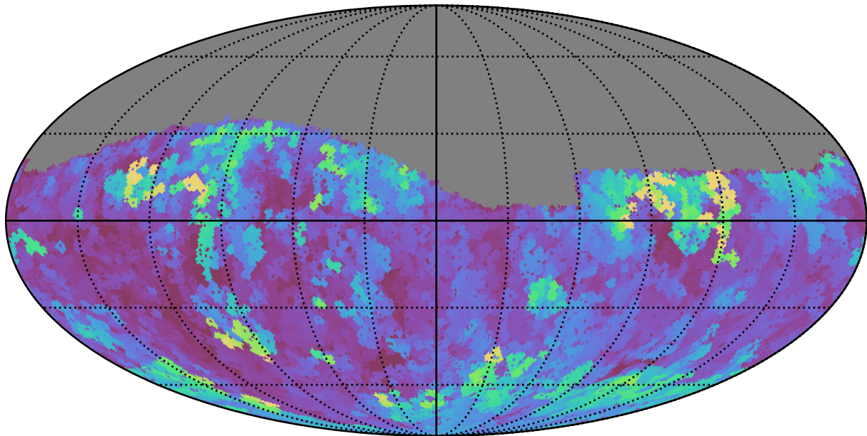
too_ignore_100_4v3.4_10yrs Yr 1 g band: Max seeingEff
