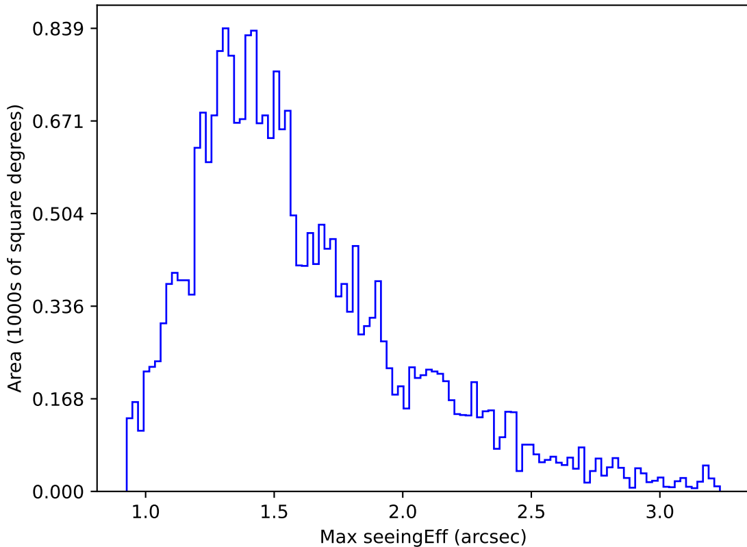
too_ignore_100_4v3.4_10yrs Yr 1 g band: Max seeingEff
